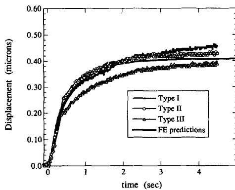
FIGURE 6 Comparison of transient displacement profiles at \rho = 5.0 for sample types I, II and III.
