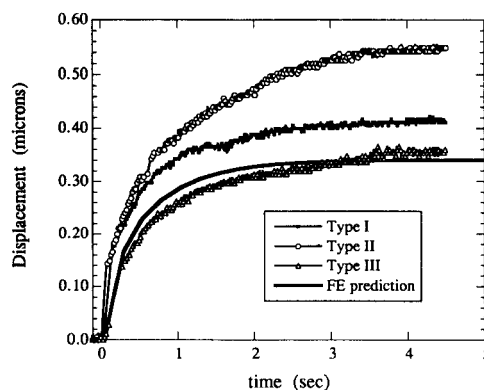
FIGURE 4 Comparison of transient displacement profiles at the fiber/matrix interface ( \rho = 1 ) for sample types I, II and III.
